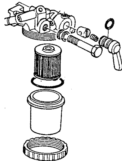
Brandstoffilter.
